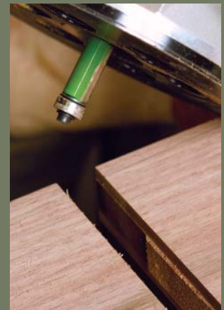
Clean up the sabersaw cut. Use a router equipped with a bearing-guided, flush-trimming bit.
